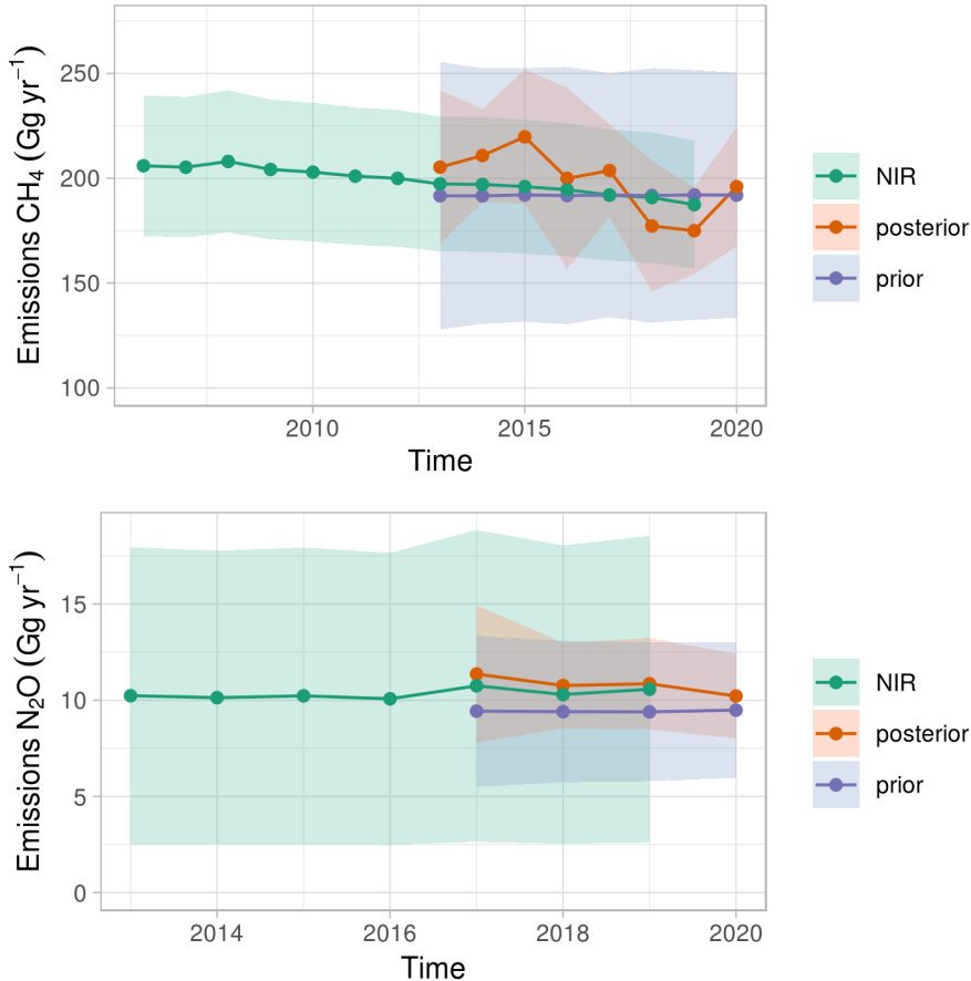
Figure S2: Chronological sequence of Swiss CH 4 emissions (above) and N 2 O emissions (below): Green, NIR; National Inventory Report) Greenhouse Gas Inventory; violet, as an a priori start value in inverse modelling; orange, as a result (a posteriori) of inverse modelling.
