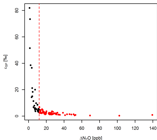
Figure 4. Standard error for SP ( \epsilon_{SP} ) of soil-derived N 2 O estimated by the Keeling plot approach as function of overnight N 2 O accumulation in the surface layer. The red dashed line shows 12 ppb increase in N 2 O mole fractions. Red dots represent the selected subset.
