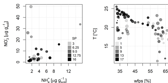
Figure 5. Maps of SP in relation to \text{NH}_4^+ and \text{NO}_3^- and SP in relation to wfps and soil temperature. The size of the points is inversely scaled to Keeling plot intercept standard error so that biggest points are those with lowest uncertainty.
